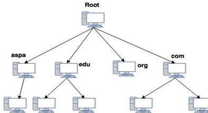
Figure 13.3 Hierarchy of DNS
