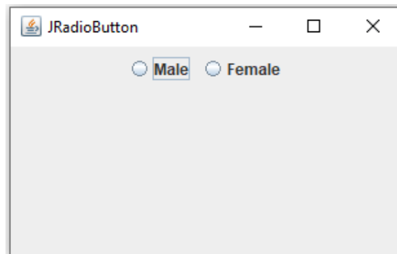
Figure 4. JRadioButton Example
