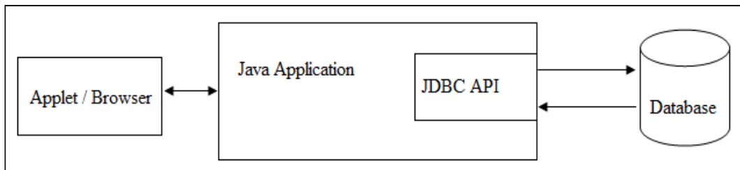
Figure 2: Three-tier Model
