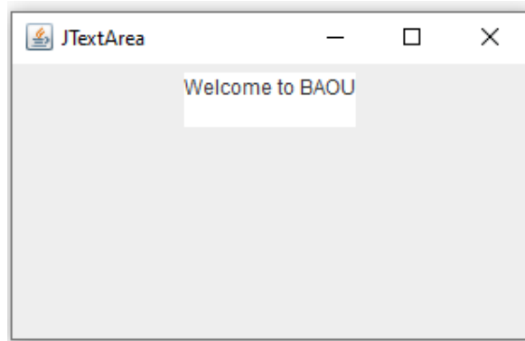
Figure 6. JTextArea Example
