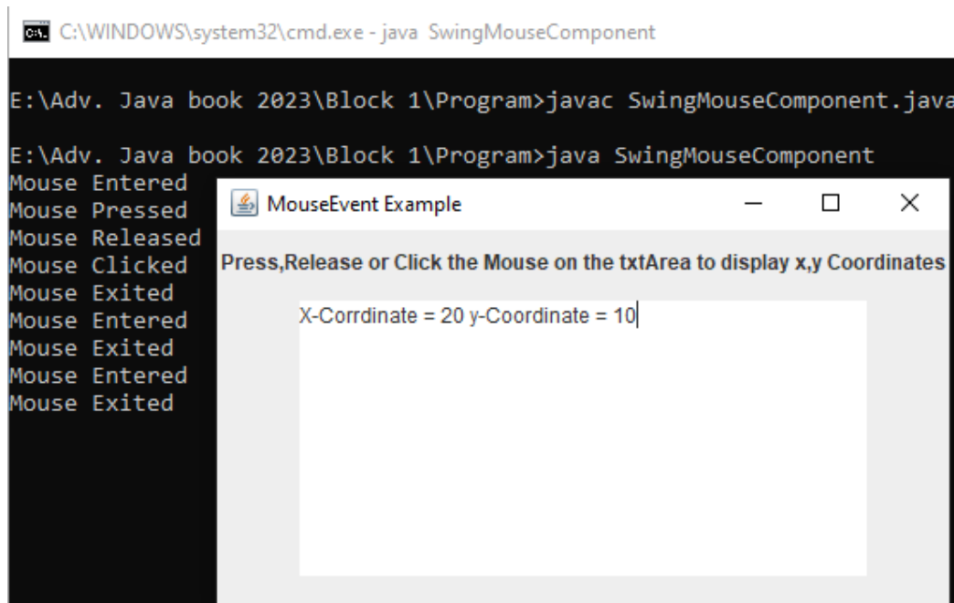
Figure 4. MouseEvent Example
