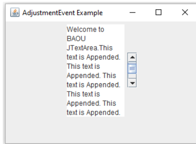
Figure 2. AdjustmentEvent Example
