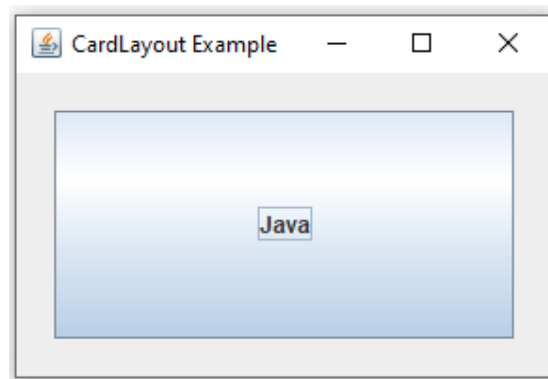
Figure 8. CardLayout Example
