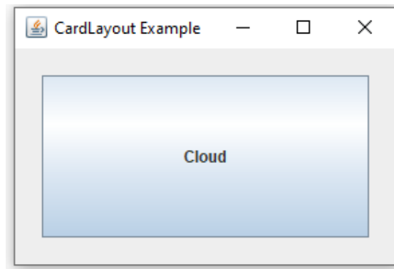
Figure 9. CardLayout Example
