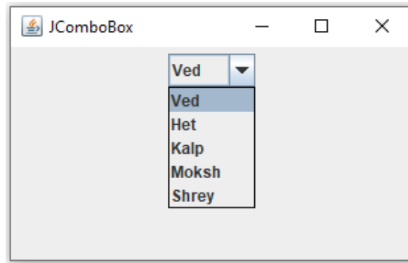
Figure 5. JComboBox Example
