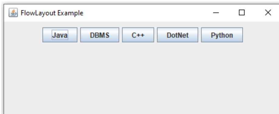
Figure 5. FlowLayout Example
