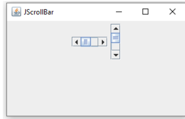
Figure 9. JScrollBar Example
