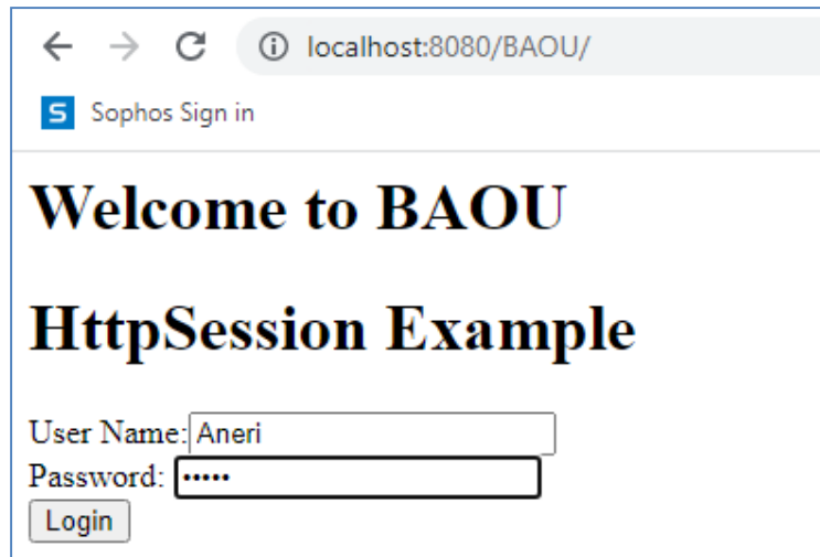
Figure 1: Welcome page
