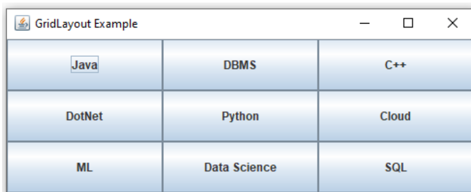
Figure 7. GridLayout Example
