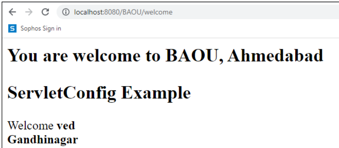
Figure 1: Use of ServletConfig to access initialization parameter
