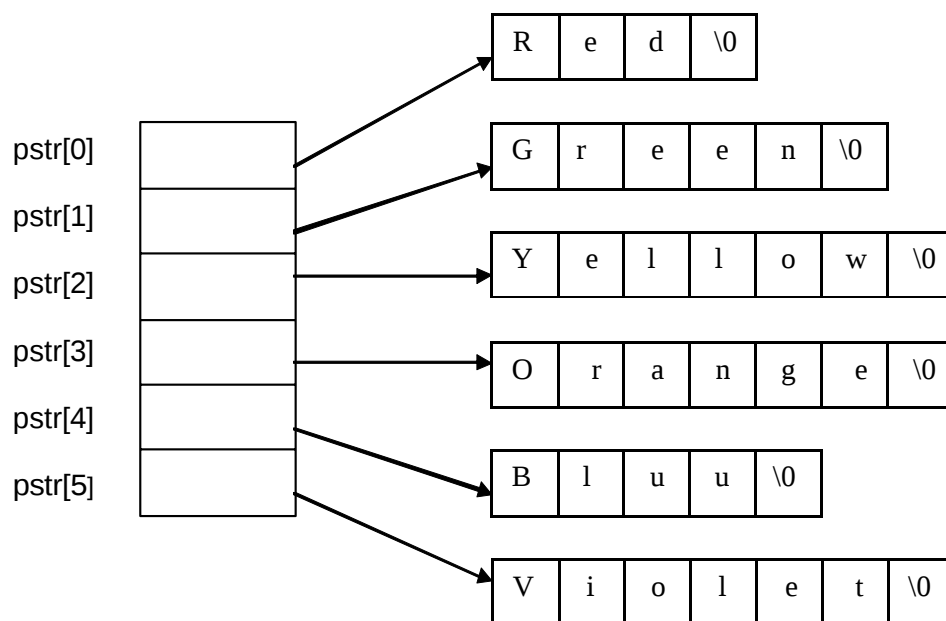
Figure 6.7 : Representation of array of pointers char *pstr[ ]
