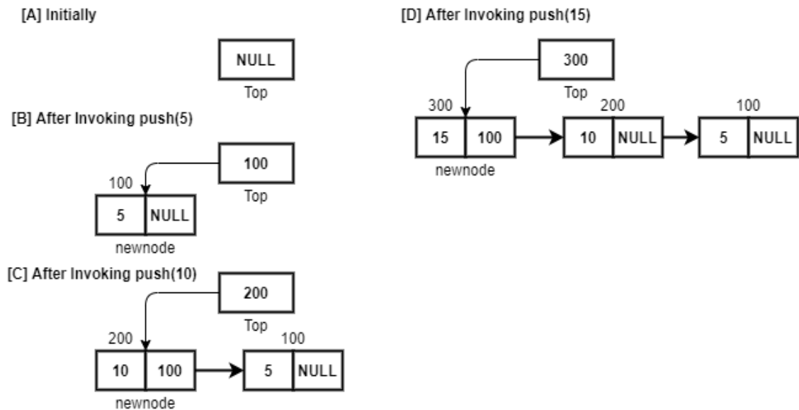
[Fig:3.3 Execution if PUSH function in the stack implemented using Link-List]
