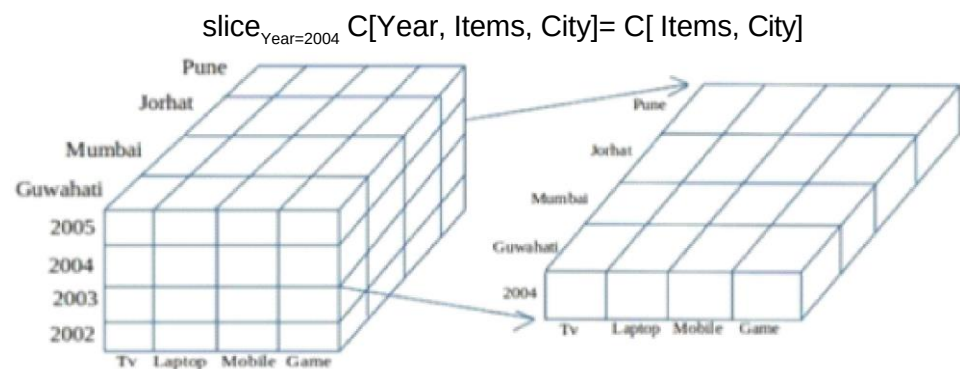
Figure 3.4: Slicing Operation
