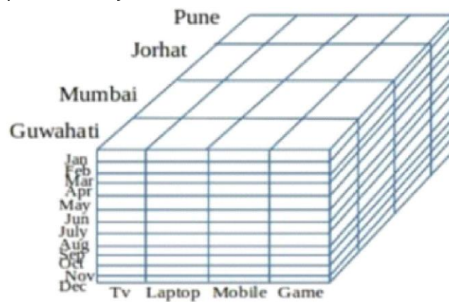
Figure 3.3: Drill-down operation
