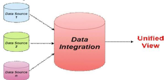
Figure 1.1: Data Integration
