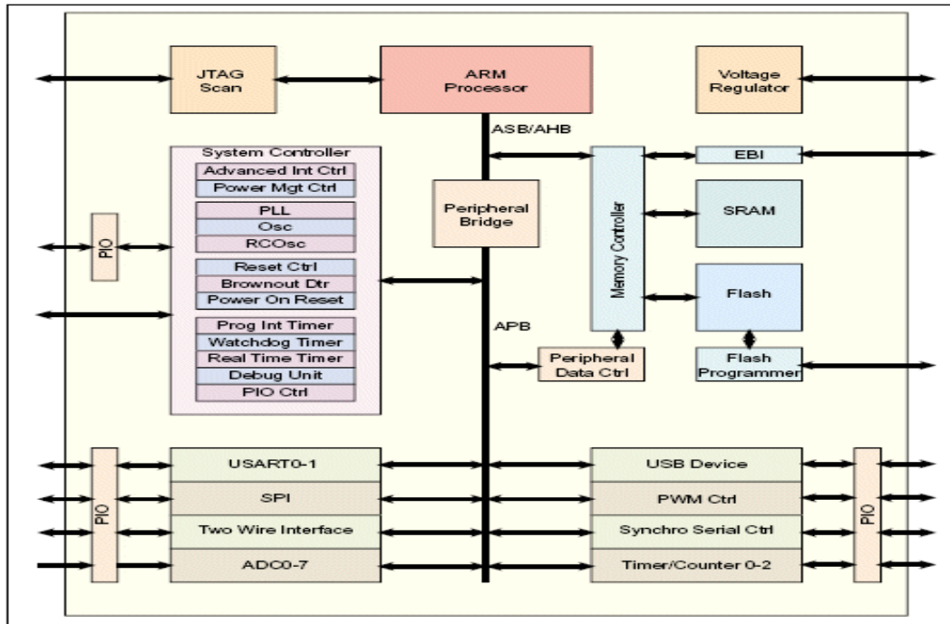
Figure-37 ARM architecture [2]
