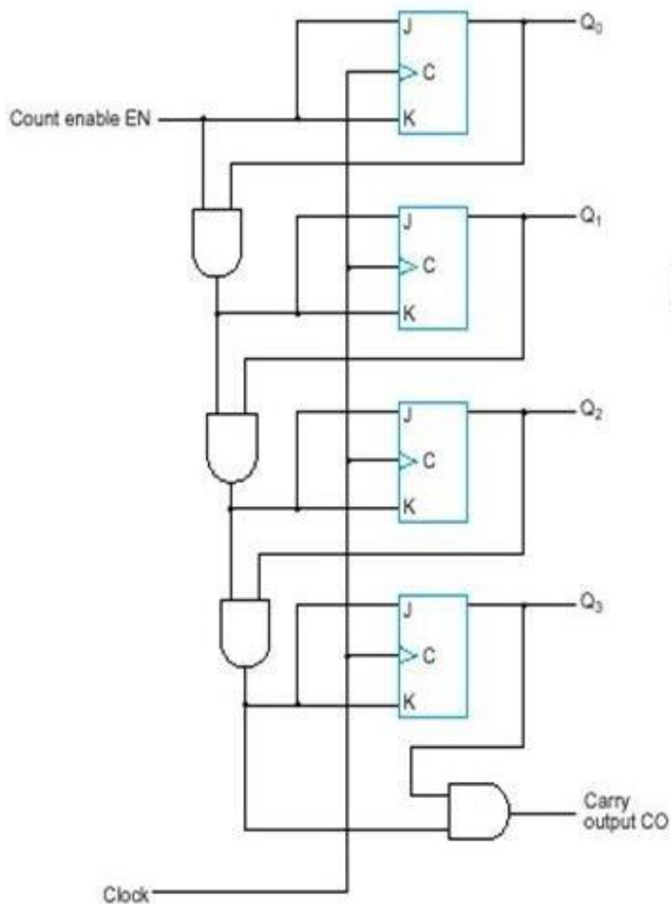
(a) Logic diagram
