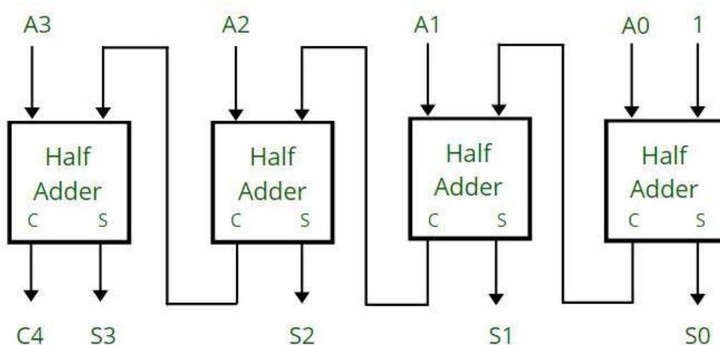
4- Bit Binary Incrementer
