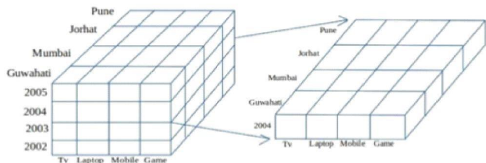
Figure 3.4: Slicing Operation
