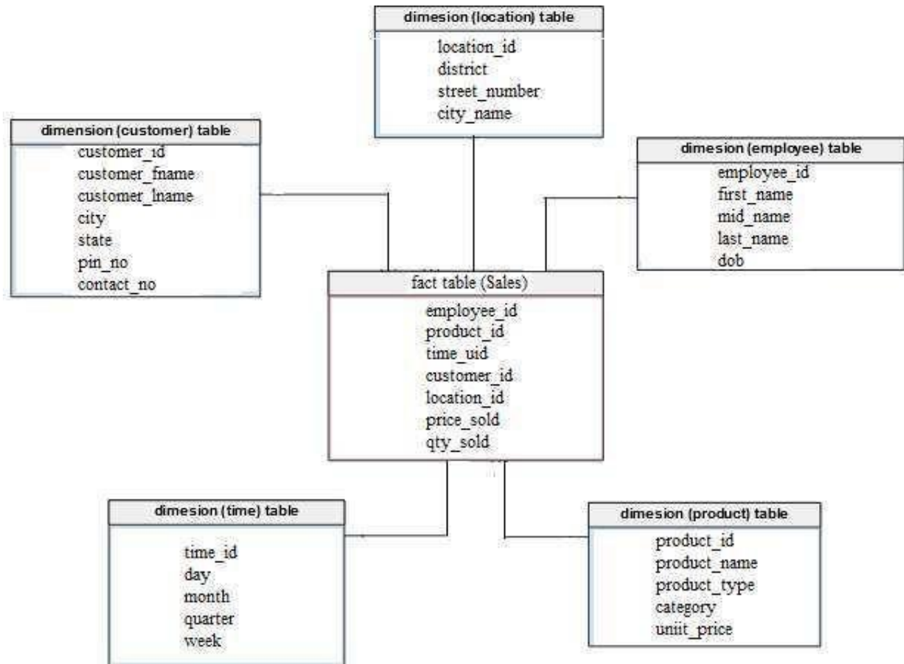
Figure 5.5: Star Schema
