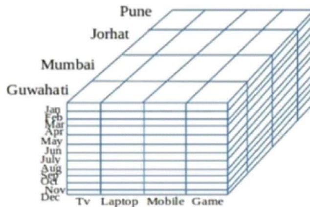
Figure 3.3: Drill-down operation
