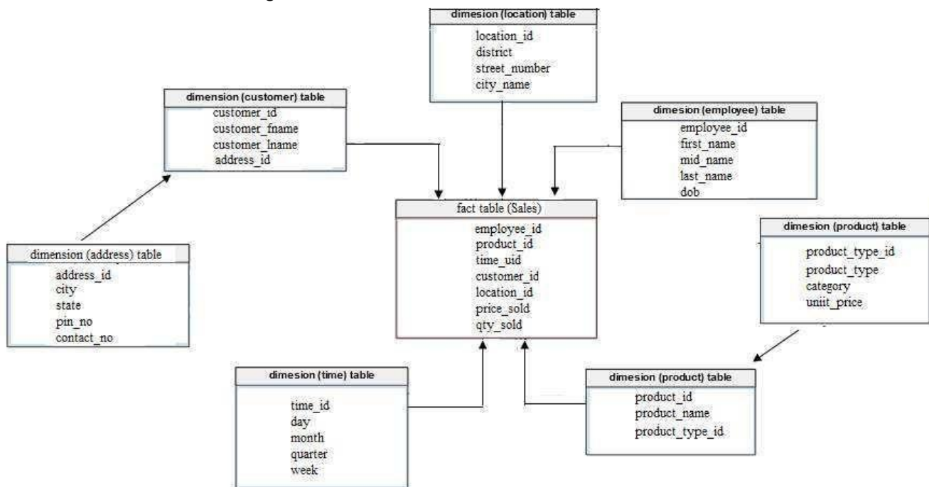
Figure 5.6: Snowflake Schema
