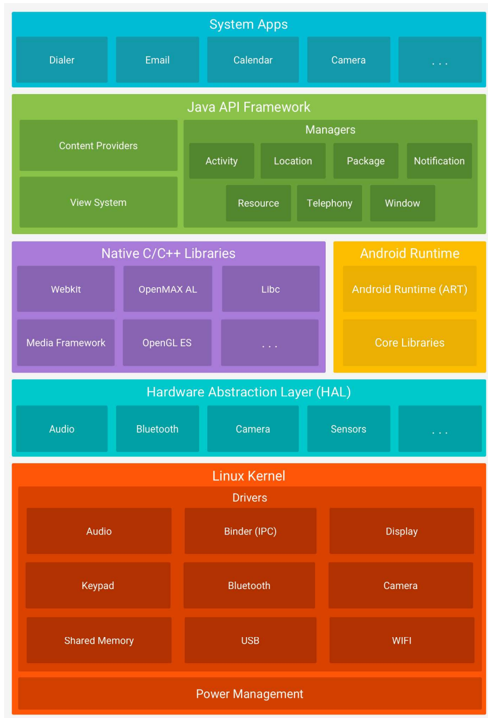
Figure-1: Android Software Stack
