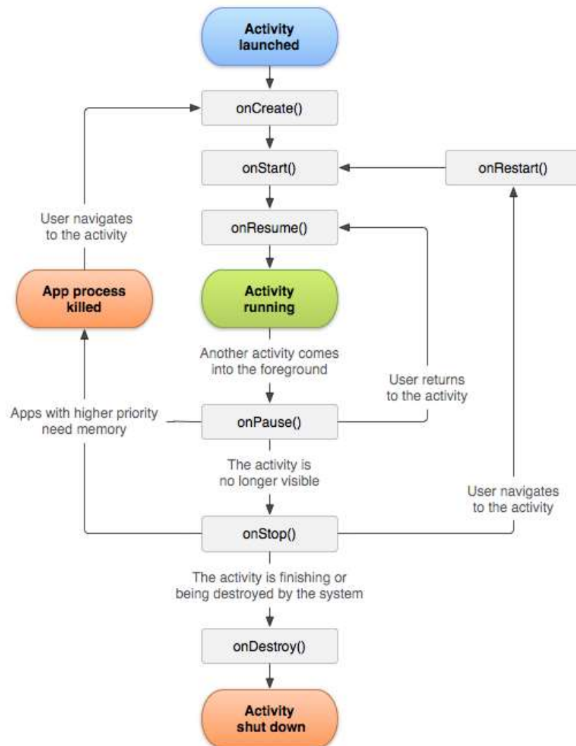
Figure-45: important state paths of an Activity
