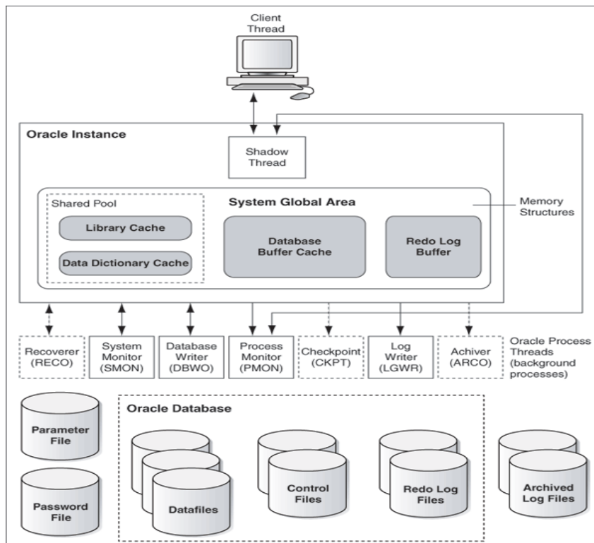
Fig. 3.1 Oracle Architecture
