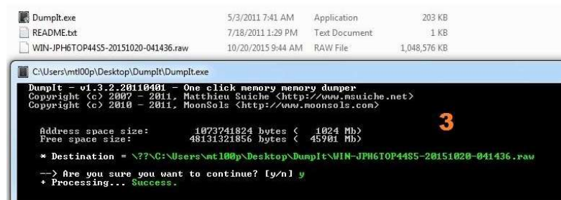
Figure 39: Command line tools for imaging
