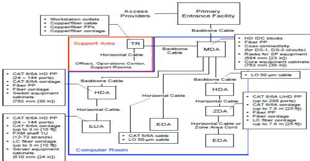
Figure 16: Cabling standards
