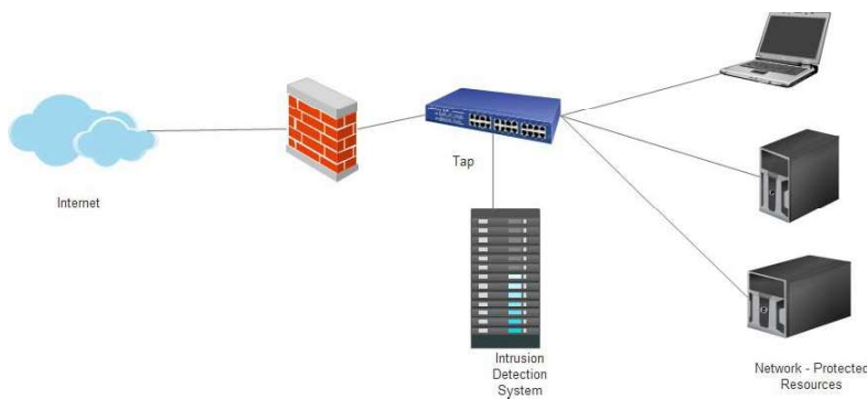
Figure 11: Placement of NBIDPS Sensors - Detection mode
