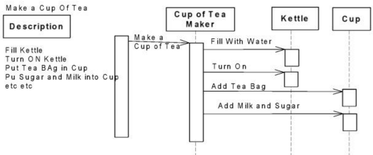
Figure: A Sequence Diagram for "Make a Cup of Tea" Use Case
